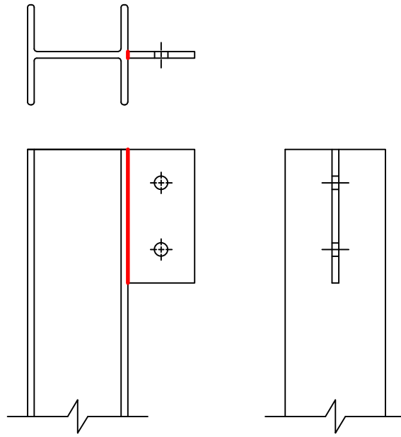
H-BEAM TYPE 2
