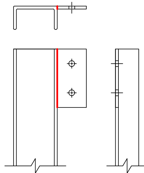
PFC TYPE 2
