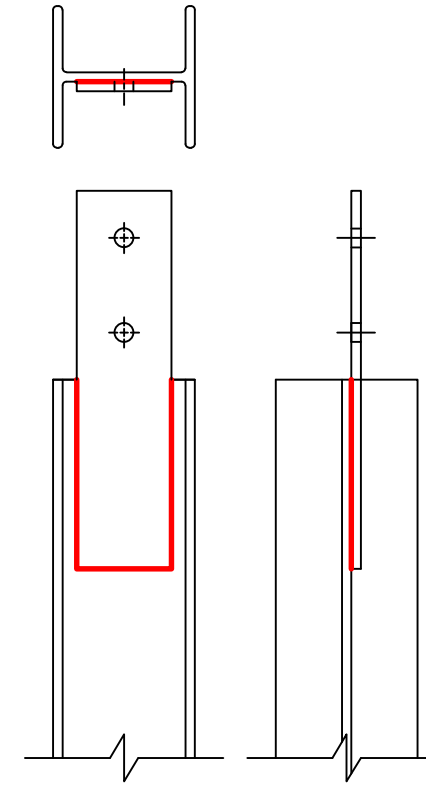
H-BEAM TYPE 3
