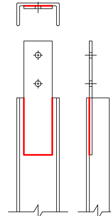
PFC TYPE 3
