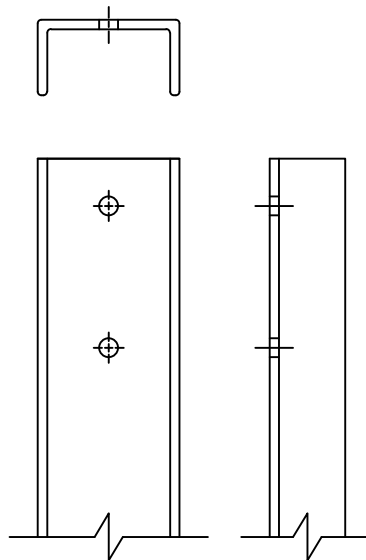
PFC TYPE 1
